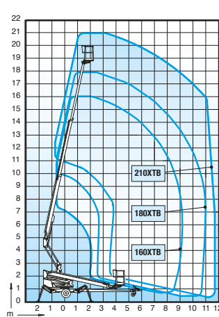
160XTB maximum outreach with 215 kg 180XTB and 210XTB maximum outreach with 80 kg
